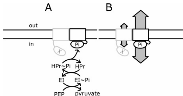
FIGURE 8: A model of the interactions between the carrier and IIA domain of LacS. The membrane-embedded carrier domain of LacS is represented by a white box to which the soluble IIA domain (represented by a white oval) is coupled via a flexible linker. The phosphorylation state of LacS-IIA is represented by X and Pi, reflecting the unphosphorylated and the phosphorylated state, respectively. The two-way arrows indicate lactose counterflow transport, and their size reflects the rate of transport. (A) Upon phosphorylation of the IIA domain by HPr(His~P) or HPr(Ser-P)-(His~P), the IIA domain interacts with the carrier domain; (B) this interaction accelerates the counterflow transport. The other subunit of the dimer (depicted in gray) is not affected by the opposing IIA domain. For clarity, only one phosphorylated subunit per dimer is shown.
