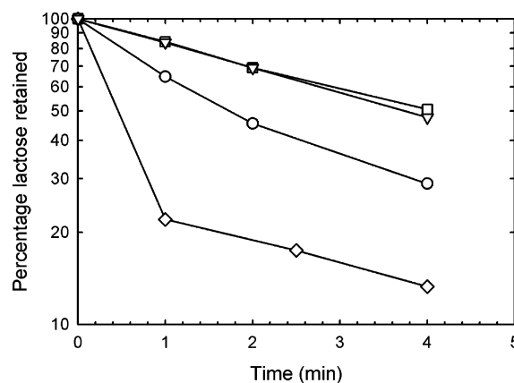
FIGURE 2: Effect of LacZ on lactose efflux by LacS. Proteoliposomes were equilibrated with 5 mM 14 C-lactose. Lactose efflux was initiated by 100-fold dilution into 50 mM KPi, pH 7.0, and 2.5% glycerol plus 5 mM MgSO 4 , yielding a final LacS concentration of 0.2 \mu M (squares). Additionally, 14 C-lactose efflux was assayed in buffers supplemented with 10 mM lactose (diamonds), 5 \mu M LacZ (circles), or 5 \mu M LacZ(E547Q) (triangles). The presence of 5 \mu M LacZ yielded a 25-fold excess of LacZ over LacS. Representative curves are shown.
