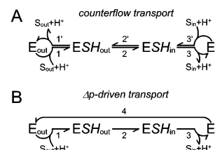
FIGURE 3: Schematic representation of counterflow and \Delta p -driven transport. E reflects the unliganded protein, ESH the fully liganded protein with both the substrate and the proton binding site occupied. S and H represent the substrate (a galactoside) and the proton, respectively. The subscripts out and in refer to the location of the binding sites, extracellular and cytoplasmic, respectively. In the wild-type protein, both the fully liganded and unliganded binding sites can reorient. (A) Lactose counterflow transport. A substrate is bound on the outside (step 1), the binding sites reorient (step 2), and the substrate is released on the inside (step 3). Next, another substrate is bound on the inside (step 3'), and reorientation to the extracellular site takes place (step 2'). Upon release of the substrate (step 1'), another round of translocation can start. Note that the counterflow mode of transport is overall an electroneutral process. The reorientation of the liganded carrier (steps 2 and 2') is proposed to be accelerated upon phosphorylation of LacS-IIA and be responsible for the increased lactose counterflow rate of phosphorylated LacS. (B) \Delta p -Driven lactose transport. Similar steps (nos. 1, 2, and 3) as described for counterflow transport take place, but upon release of the substrate on the inside (step 3), substrate is not bound on the trans side. Rather, the unliganded binding site reorients to the outside (step 4) and initiates another round of translocation.
